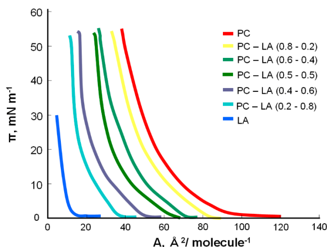
Figure 3. Surface pressure–area ( \pi -A) isotherms of mixed PC–LA monolayer.
