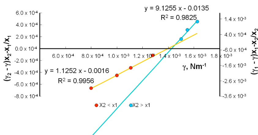
Figure 12. A plot showing Equations (17) and (18) for determining B_1 , B_2 , and \gamma : parameters of the PC–LA system.
