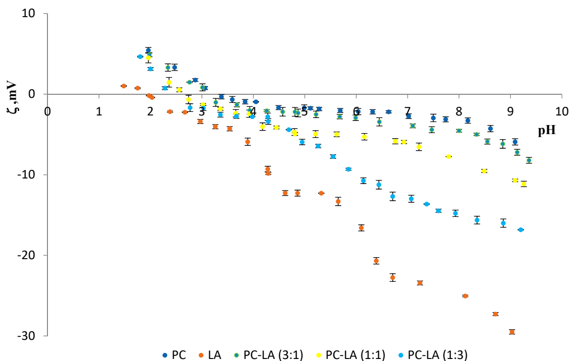
Figure 7. Dependence of PC and PC: LA membrane zeta potential values vs. the pH of the electrolyte solution.
