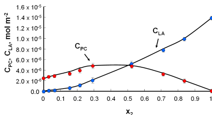
Figure 4. Dependence of the total surface concentration of PC ( c_{PC} ) and LA ( c_{LA} ) vs. the mole fraction of LA (the experimental values are indicated by the points and the theoretical values by the curve).
