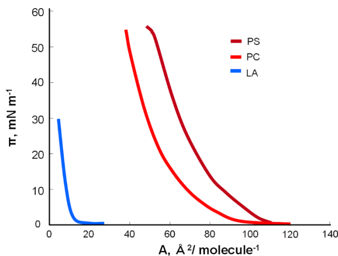
Figure 2. \pi -A isotherms of phosphatidylcholine (PC), phosphatidylserine (PS), and lipoic acid (LA).
