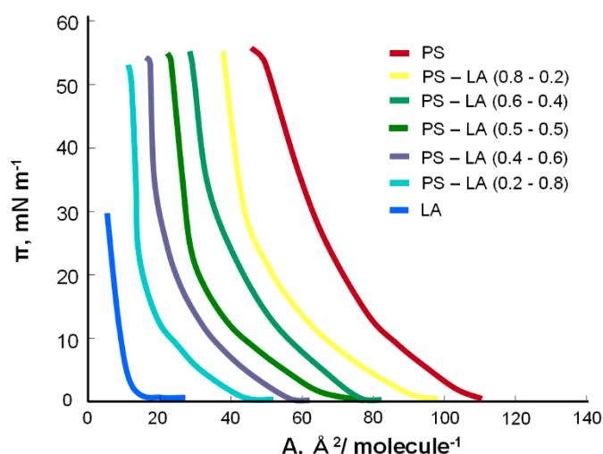
Figure 5. Surface pressure–area ( \pi -A) isotherms of the mixed PS–LA monolayers.
